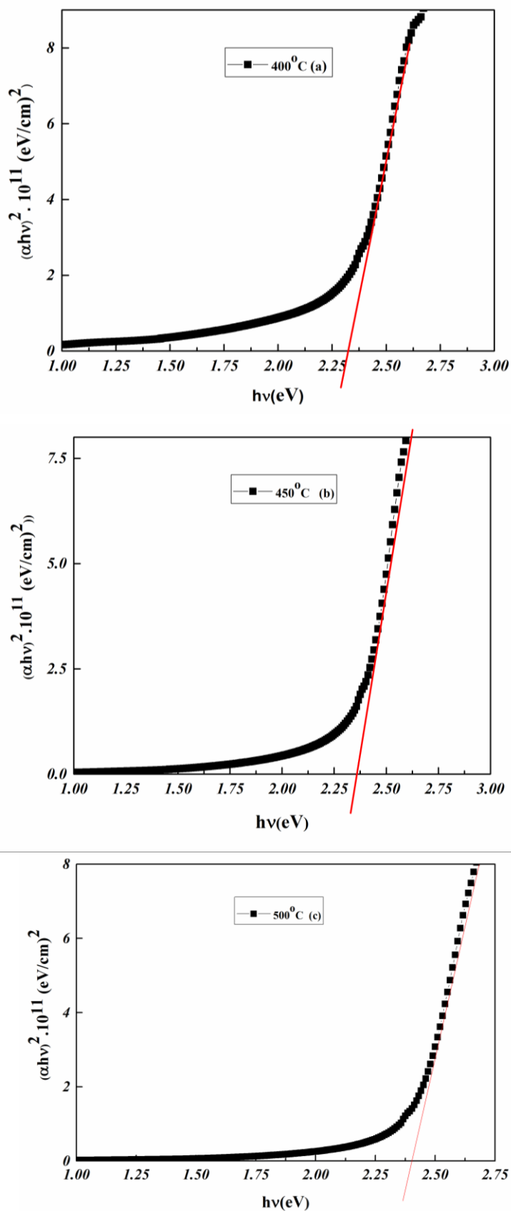
Fig.5 (a, b, c) relation between (\alpha h\nu)^2 and h\nu for (\text{V}_2\text{O}_5) thin films prepared at different substrate temperatures.
