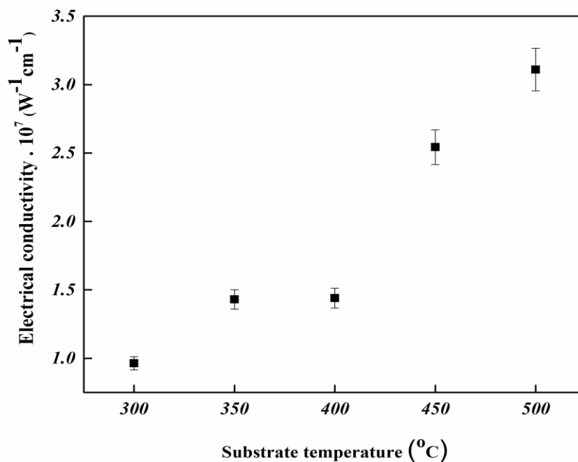
Fig.3 Electrical conductivity of (V 2 O 5 ) thin film deposited at different temperatures.
