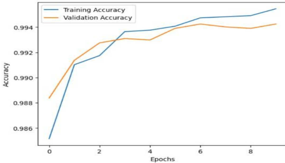
Fig.8. Model_accuracy
